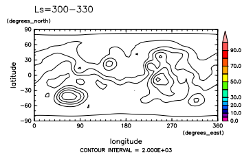
Figure 375: Prec. water at 14 LST and Ls=270°-300° by DCPAM
