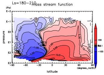
Figure 142: MSF at L_S=180^\circ-210^\circ by DCPAM
