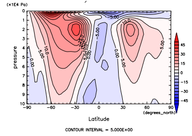
Figure 232: U at Jun. by DCPAM
