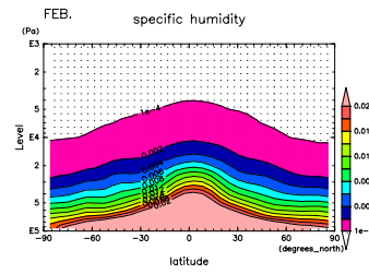
Figure 724: q at Feb. by DCPAM
