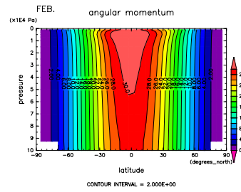
Figure 253: ANGMOM at Jan. by DCPAM by Figure 256: ANGMOM at Feb. by DCPAM
