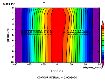
Figure 253: ANGMOM at Jan. by DCPAM by Figure 256: ANGMOM at Feb. by DCPAM
