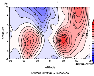
Figure 542: U at Jan. by NCEP
