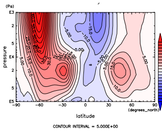
Figure 566: U at Sep. by NCEP
