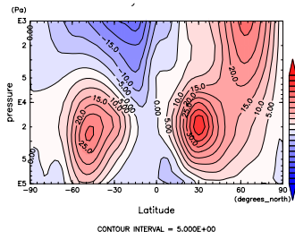
Figure 541: U at Jan. by DCPAM
