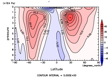
Figure 223: U at Mar. by DCPAM
