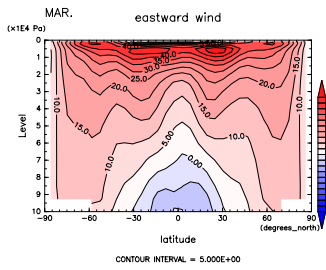
Figure 223: U at Mar. by DCPAM
