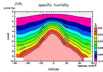
Figure 412: q at Jun. by DCPAM
