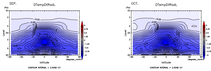
Figure 849: (\partial T/\partial t)_{LW} at Sep. by DCPAM Figure 850: (\partial T/\partial t)_{LW} at Oct. by DCPAM
