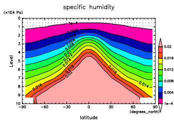
Figure 34: Annual mean q by DCPAM
