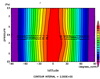
Figure 578: ANG MOM at Jan. by NCEP by Figure 581: ANG MOM at Feb. by NCEP
