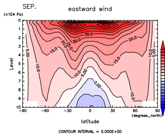
Figure 241: U at Sep. by DCPAM
