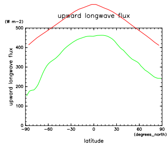
Figure 7: Annual average SLURA by DCPAM (red), NCEP (green)
