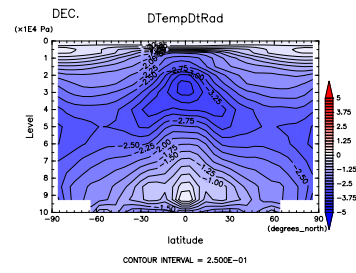
Figure 540: (\partial T / \partial t)_{SW+LW} at Dec. by DCPAM
