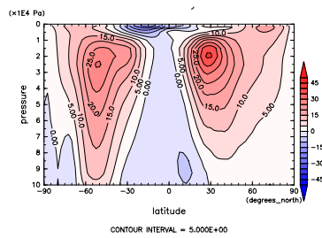
Figure 224: U at Mar. by NCEP
