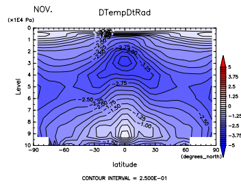
Figure 539: (\partial T / \partial t)_{SW+LW} at Nov. by DCPAM
