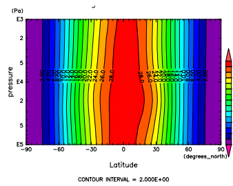
Figure 577: ANG MOM at Jan. by DCPAM by Figure 580: ANG MOM at Feb. by DCPAM
