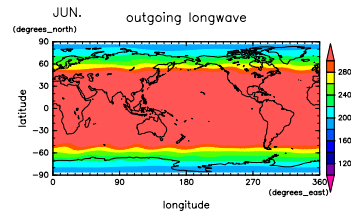
Figure 136: OLR at Jun. by DCPAM
