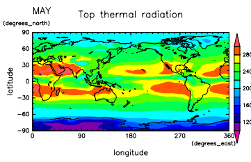
Figure 134: OLR at May by NCEP
