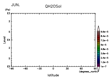
Figure 810: q_i at Jun. by DCPAM
