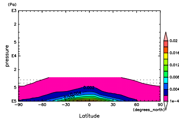
Figure 754: q at Dec. by DCPAM
