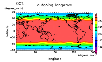
Figure 145: OLR at Sep. by DCPAM Figure 148: OLR at Oct. by DCPAM
