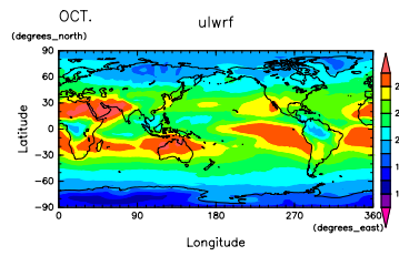
Figure 145: OLR at Sep. by DCPAM Figure 148: OLR at Oct. by DCPAM
