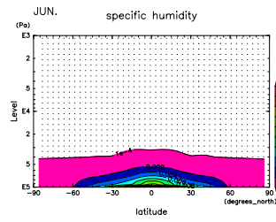
Figure 736: q at Jun. by DCPAM
