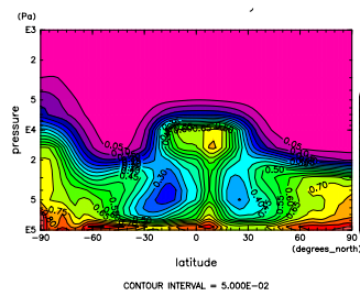
Figure 785: RH at Oct. by NCEP
