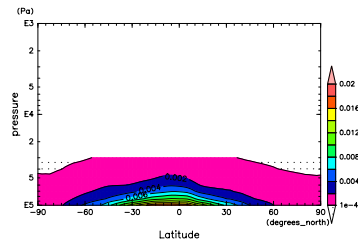
Figure 724: q at Feb. by DCPAM
