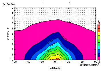
Figure 428: q at Nov. by NCEP
