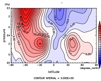
Figure 557: U at Jun. by NCEP
