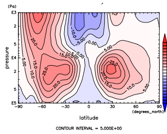
Figure 551: U at Apr. by NCEP
