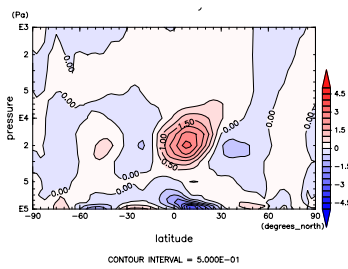
Figure 614: V at Jan. by NCEP
