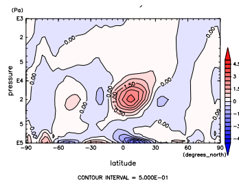
Figure 617: V at Feb. by NCEP
