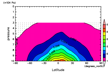
Figure 424: q at Oct. by DCPAM
