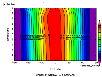
Figure 278: ANGMOM at Sep. by NCEP by Figure 281: ANGMOM at Oct. by NCEP
