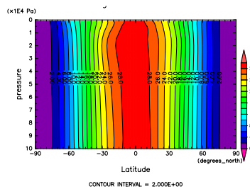
Figure 277: ANGMOM at Sep. by DCPAM by Figure 280: ANGMOM at Oct. by DCPAM
