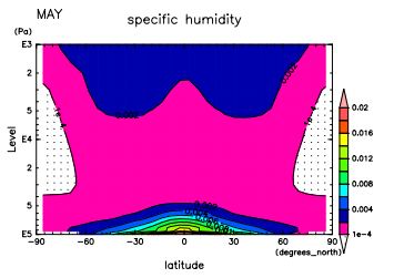
Figure 733: q at May by DCPAM
