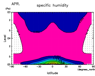
Figure 730: q at Apr. by DCPAM
