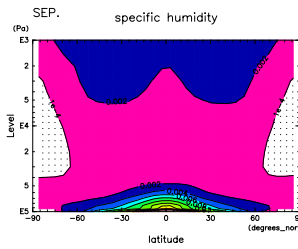
Figure 745: q at Sep. by DCPAM
