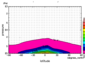
Figure 752: q at Nov. by NCEP
