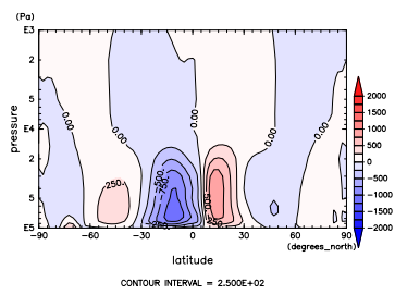
Figure 56: Annual mean MSF by NCEP
