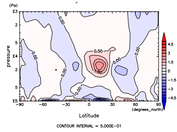
Figure 646: V at Dec. by DCPAM
