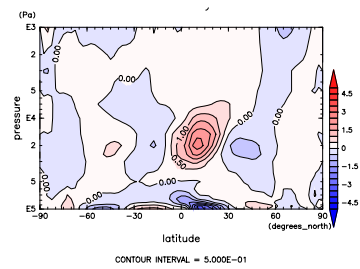
Figure 647: V at Dec. by NCEP
