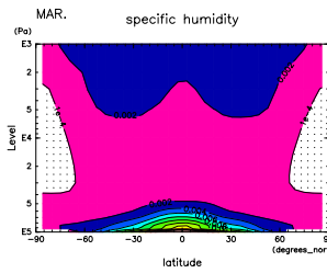
Figure 727: q at Mar. by DCPAM
