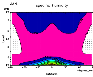
Figure 721: q at Jan. by DCPAM
