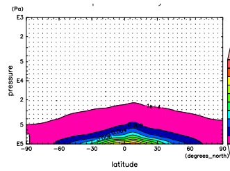
Figure 749: q at Oct. by NCEP
