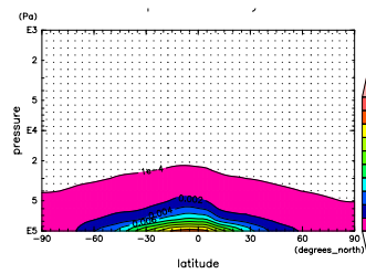
Figure 725: q at Feb. by NCEP
