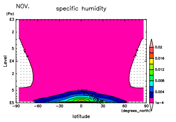
Figure 751: q at Nov. by DCPAM
