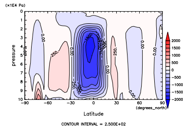
Figure 346: MSF at Aug. by DCPAM
