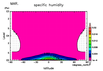
Figure 727: q at Mar. by DCPAM
