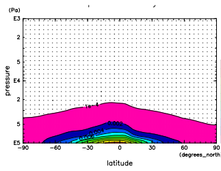
Figure 722: q at Jan. by NCEP
