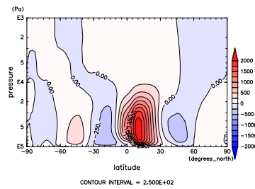
Figure 683: MSF at Dec. by NCEP
