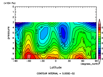
Figure 436: RH at Feb. by DCPAM
