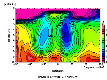
Figure 437: RH at Feb. by NCEP
