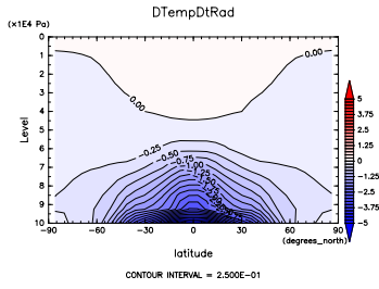
Figure 45: Annual mean (\partial T / \partial t)_{SW+LW} by DCPAM
