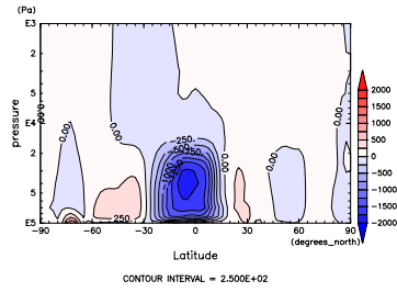
Figure 670: MSF at Aug. by DCPAM
