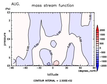
Figure 670: MSF at Aug. by DCPAM
