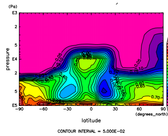
Figure 761: RH at Feb. by NCEP
