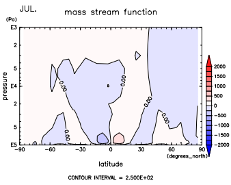
Figure 667: MSF at Jul. by DCPAM
