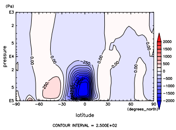
Figure 668: MSF at Jul. by NCEP
