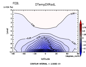
Figure 518: (\partial T/\partial t)_{LW} at Feb. by DCPAM
