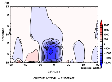
Figure 667: MSF at Jul. by DCPAM
