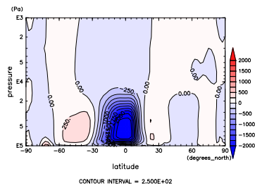
Figure 671: MSF at Aug. by NCEP
