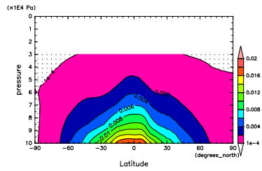
Figure 406: q at Apr. by DCPAM
