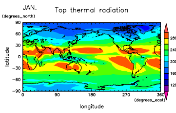
Figure 122: OLR at Jan. by NCEP
