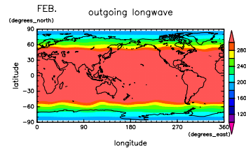
Figure 124: OLR at Feb. by DCPAM
