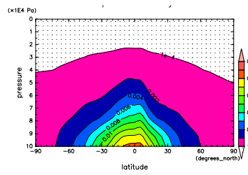
Figure 431: q at Dec. by NCEP
