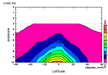
Figure 430: q at Dec. by DCPAM
