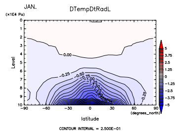
Figure 517: (\partial T/\partial t)_{LW} at Jan. by DCPAM
