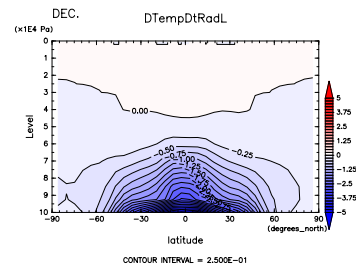
Figure 528: (\partial T / \partial t)_{LW} at Dec. by DCPAM
