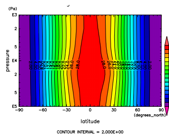
Figure 587: ANGMOM at Apr. by NCEP
