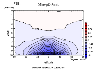
Figure 518: (\partial T/\partial t)_{LW} at Feb. by DCPAM
