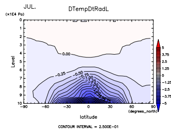
Figure 523: (\partial T / \partial t)_{LW} at Jul. by DCPAM
