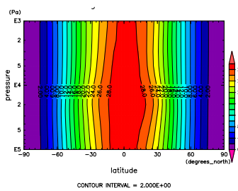
Figure 584: ANGMOM at Mar. by NCEP
