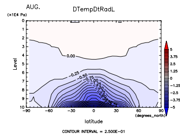
Figure 524: (\partial T / \partial t)_{LW} at Aug. by DCPAM
