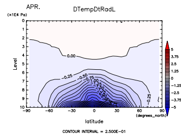
Figure 520: (\partial T/\partial t)_{LW} at Apr. by DCPAM
