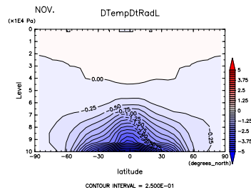
Figure 527: (\partial T / \partial t)_{LW} at Nov. by DCPAM
