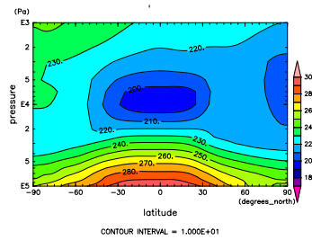
Figure 689: T at Feb. by NCEP
