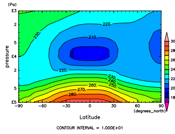
Figure 688: T at Feb. by DCPAM
