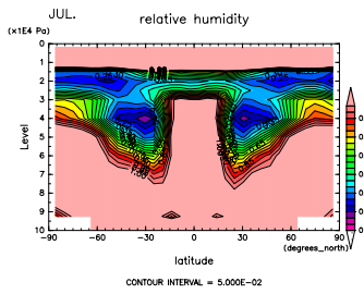
Figure 451: RH at Jul. by DCPAM
