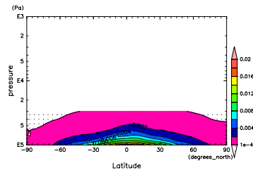
Figure 748: q at Oct. by DCPAM
