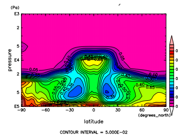
Figure 767: RH at Apr. by NCEP
