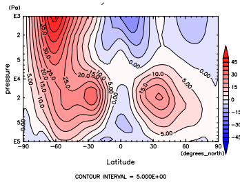
Figure 553: U at May by DCPAM
