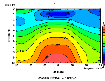
Figure 395: T at Dec. by NCEP
