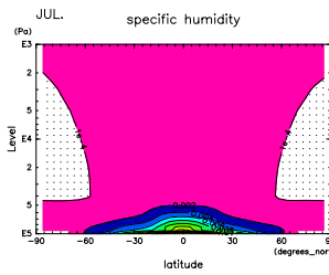
Figure 739: q at Jul. by DCPAM
