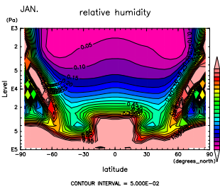
Figure 757: RH at Jan. by DCPAM
