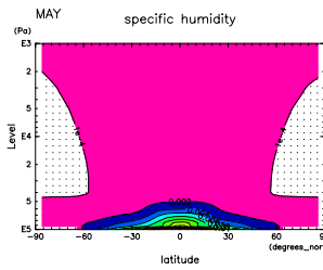
Figure 733: q at May by DCPAM
