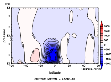
Figure 662: MSF at May by NCEP Figure 665: MSF at Jun. by NCEP
