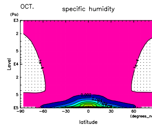
Figure 748: q at Oct. by DCPAM
