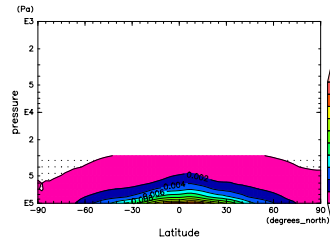
Figure 748: q at Oct. by DCPAM
