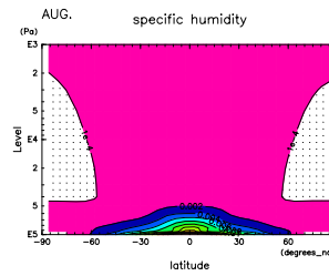
Figure 742: q at Aug. by DCPAM
