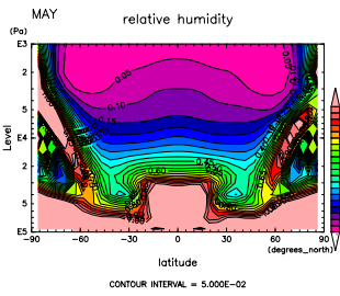
Figure 769: RH at May by DCPAM
