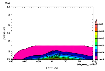
Figure 742: q at Aug. by DCPAM
