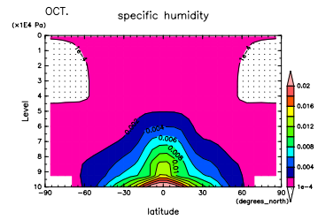
Figure 424: q at Oct. by DCPAM
