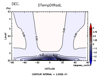
Figure 852: (\partial T/\partial t)_{LW} at Dec. by DCPAM
