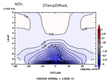
Figure 527: (\partial T/\partial t)_{LW} at Nov. by DCPAM
