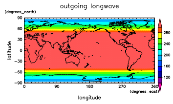
Figure 11: Annual mean OLR by DC-PAM
