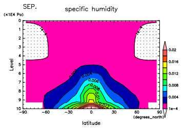
Figure 421: q at Sep. by DCPAM
