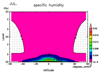
Figure 739: q at Jul. by DCPAM
