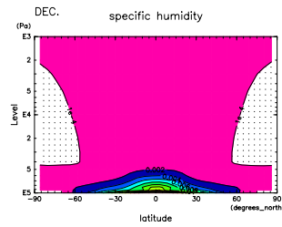
Figure 754: q at Dec. by DCPAM
