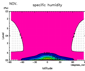
Figure 751: q at Nov. by DCPAM
