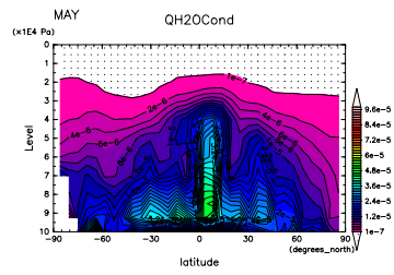
Figure 497: q_l + q_s at May by DCPAM Figure 498: q_l + q_s at Jun. by DCPAM
