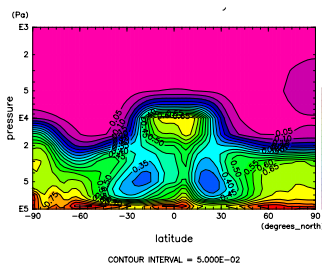
Figure 788: RH at Nov. by NCEP
