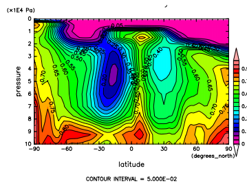
Figure 452: RH at Jul. by NCEP
