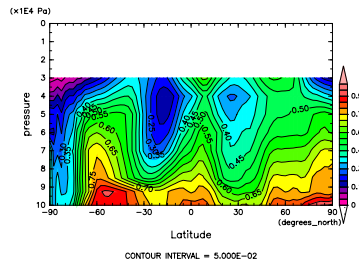
Figure 451: RH at Jul. by DCPAM
