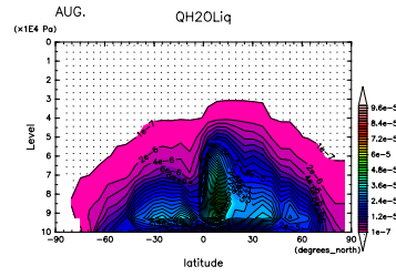
Figure 476: q_l at Aug. by DCPAM
