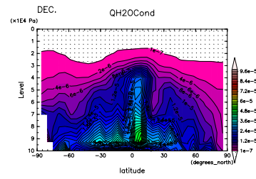
Figure 503: q_l + q_i at Nov. by DCPAM Figure 504: q_l + q_i at Dec. by DCPAM
