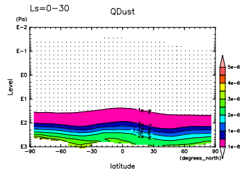
Figure 208: QDust at L_S=0^\circ-30^\circ by DCPAM
