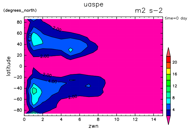
Figure 8: Spectrum of zonal wind by DCPAM
