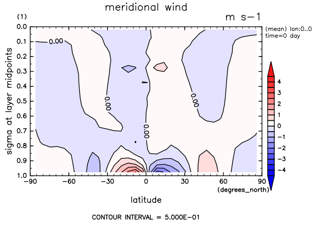
Figure 2: Zonal mean meridional wind by DCPAM
