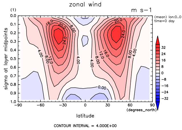
Figure 1: Zonal mean zonal wind by DCPAM
