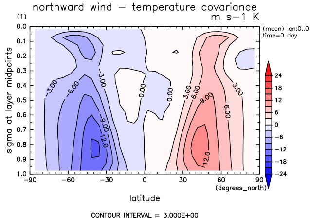
Figure 6: Zonal mean meridional wind and temperature covariance by DCPAM
