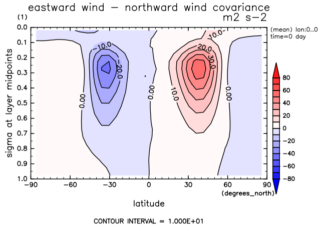
Figure 7: Zonal mean zonal wind and meridional wind covariance by DCPAM
