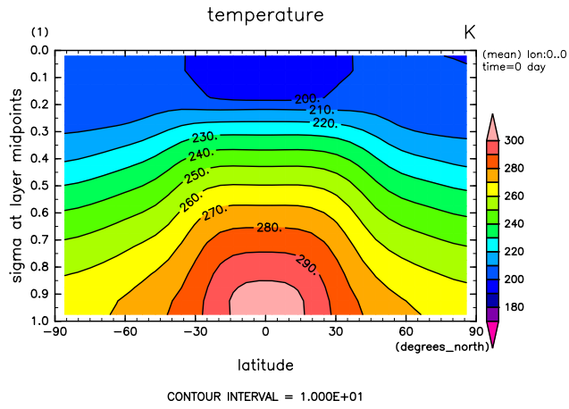
Figure 4: Zonal mean temperature by DCPAM
