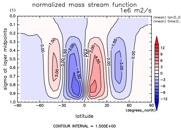
Figure 3: Normalized mass stream function by DCPAM
