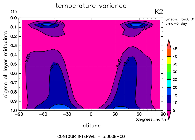
Figure 5: Zonal mean zonal eddy temperature squared by DCPAM
