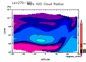
Figure 205: H 2 O cloud radius at L s =270°–300° by DCPAM
